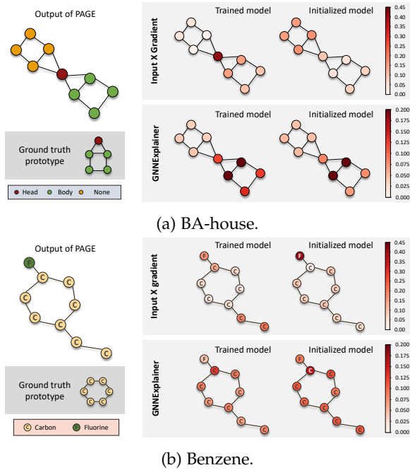
Fig. 9: Visualization of the attribution score as a heatmap where \text{Input} \times \text{Gradient} and \text{GNNExplainer} are adopted to the output prototype graphs from PAGE for the BA-house and Benzene datasets.
